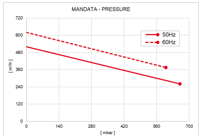
Curve riferite alla pressione di 1013mbar (Ass.) e temperatura 20°C (tolleranza \pm 10%) Curves refer to 1013mbar (Abs.) pression and 20°C temperature (tolerance \pm 10%)
